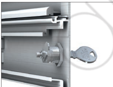
Cylinder cutout provided by the customer for the master key system cylinder being delivered
